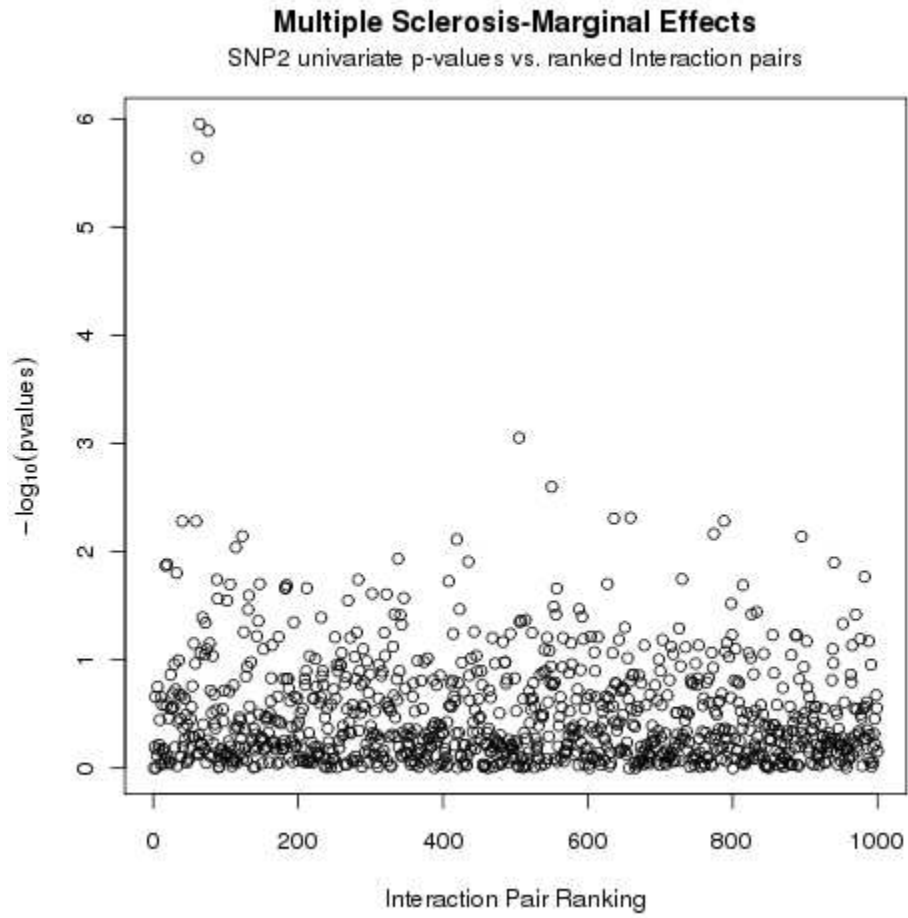
Figure.S 5: Multiple Sclerosis SNP2 univariate P-values versus EPIBLASTER interaction pair ranking for top 1000 pairs.
