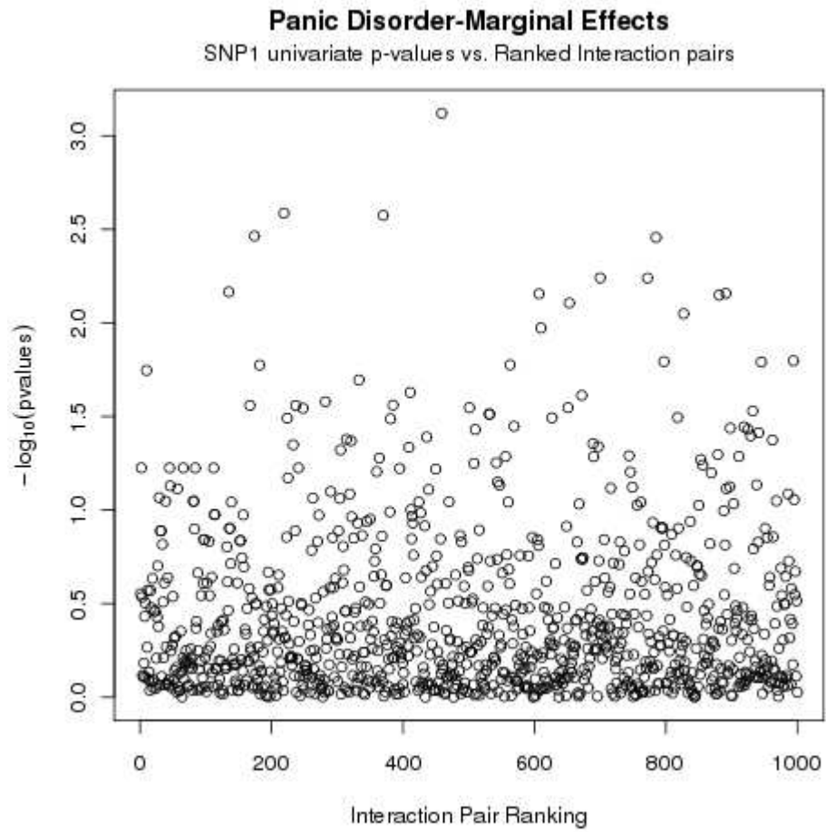
Figure.S 2: Panic Disorder SNP1 univariate P-values versus EPIBLASTER interaction pair ranking for top 1000 pairs.
