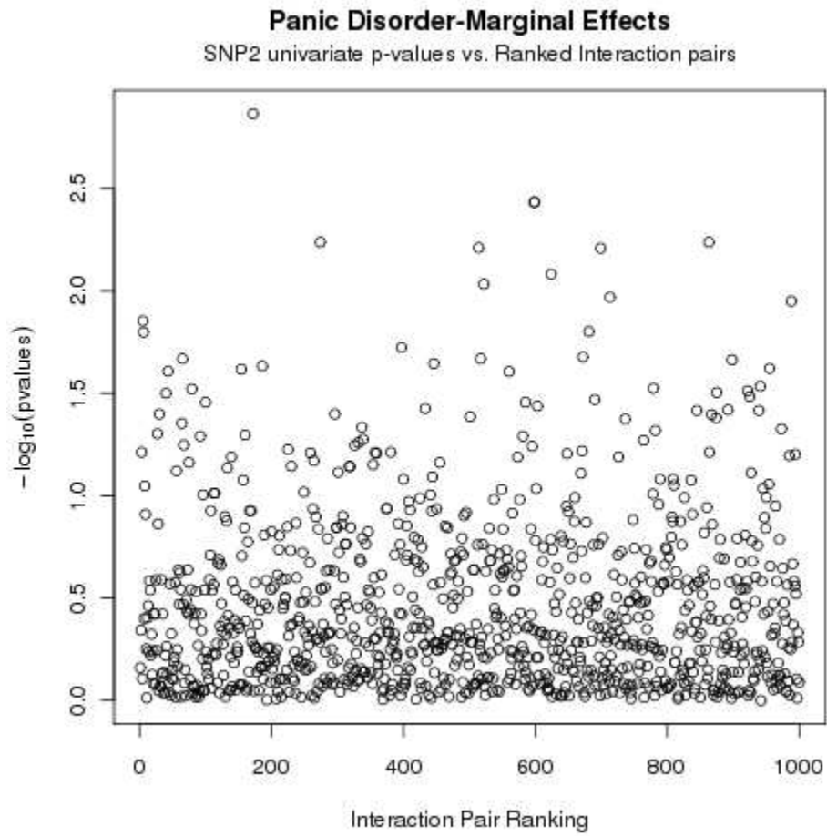
Figure.S 3: Panic Disorder SNP2 univariate P-values versus EPIBLASTER interaction pair ranking for top 1000 pairs.
