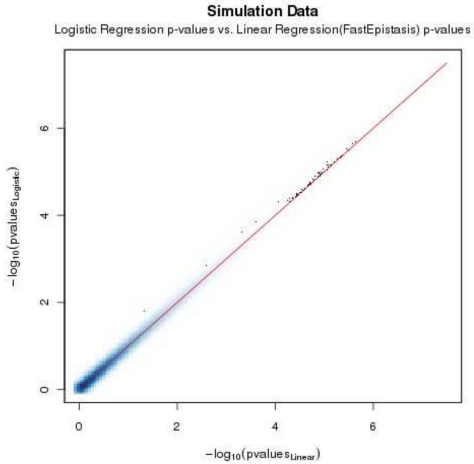
Figure.S 1. Logarithmic p-values from interaction term of the logistic regression model versus linear regression model. ( R^2=99.9\% ). Red line marks unit slope line.
