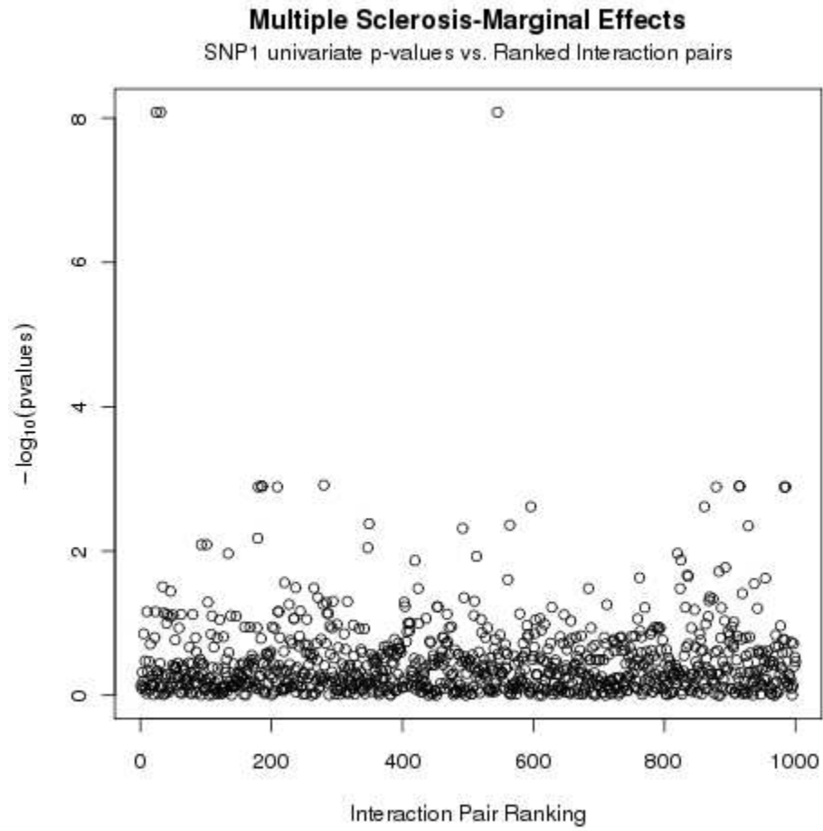
Figure.S 4: Multiple Sclerosis SNP1 univariate P-values versus EPIBLASTER interaction pair ranking for top 1000 pairs.
