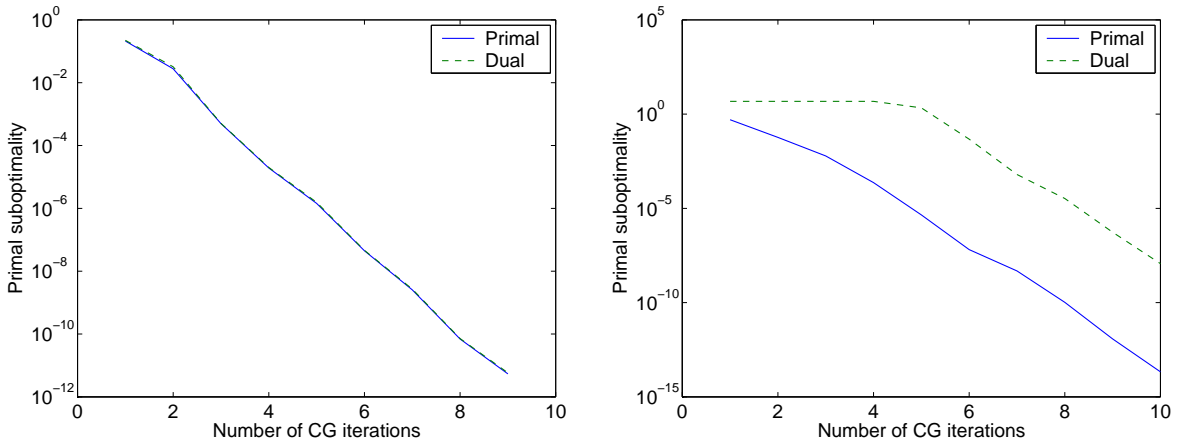
Figure 1: Plots of the primal suboptimality, (2)-(3), for primal and dual optimization by conjugate gradient (pcg in Matlab). n points are drawn randomly from a spherical Gaussian distribution in d dimensions. The targets are also randomly generated according a Gaussian distribution. \lambda is fixed to 1. Left, n = 10 and d = 100 . Right, n = 100 and d = 10 .
