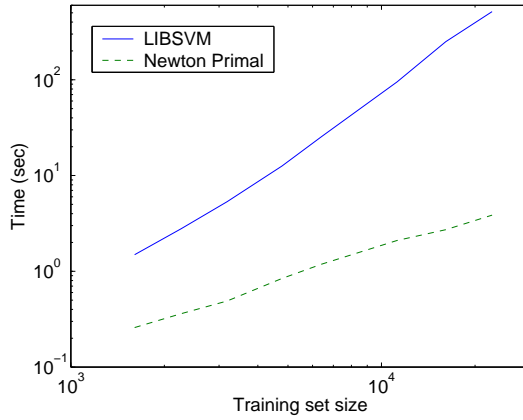
Figure 4: Time comparison of LIBSVM (an implementation of SMO [Platt, 1998]) and direct Newton optimization on the normal vector w .
